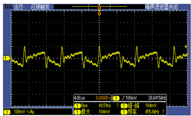
Figure 7, Output ripple & noise ( I_{out} = 10\text{A} )
