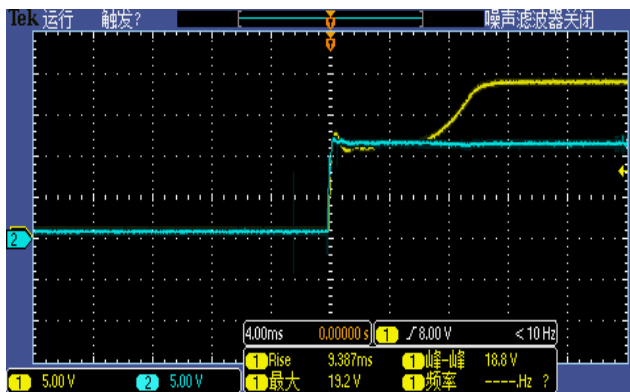
Figure 6, Output voltage established ( I_{out} = 10\text{A} )
