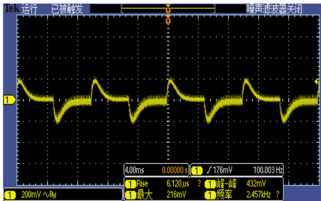
Figure 4, 25% - 50% load dynamic
