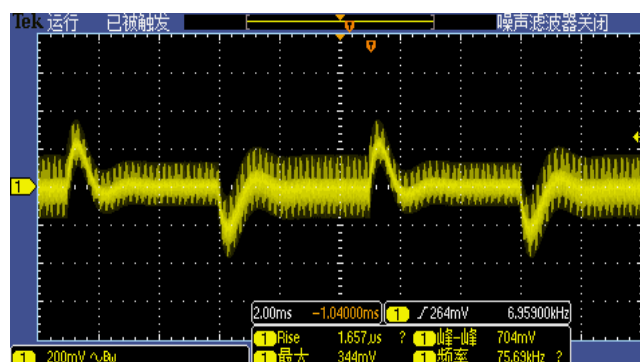
Figure 5, 50% - 75% load dynamic
