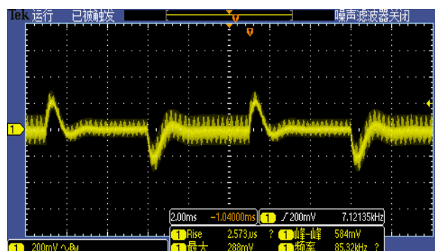
Figure 4, 25% - 50% load dynamic
