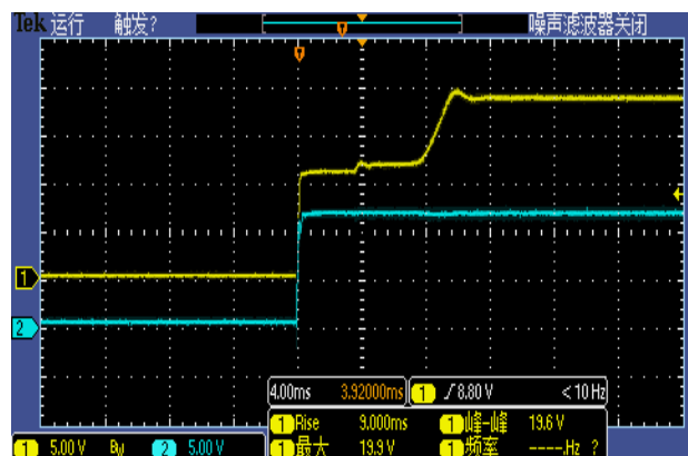
Figure 6, Output voltage established ( I_{out} = 3\text{A} )
