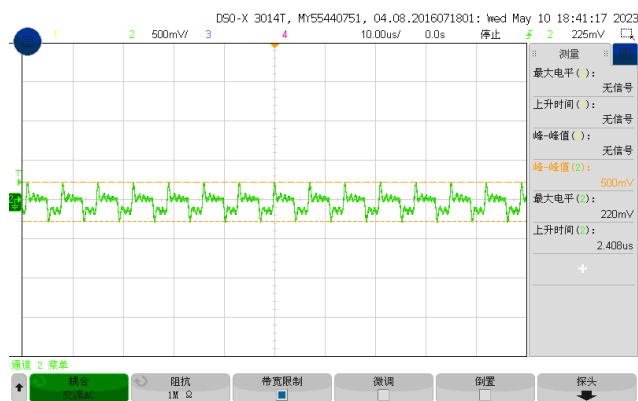
Figure 7, Output ripple & noise ( I_{out} = 5\text{A} )
