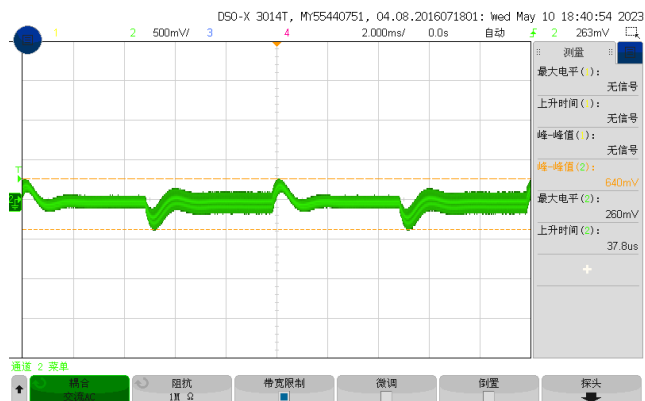
Figure 4, 25% - 50% load dynamic
