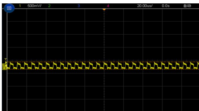
Figure 7, Output ripple & noise ( I_{out} = 1\text{A} )
