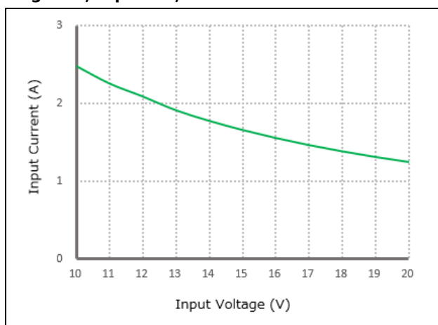
Figure 3, Input V-I, I_{out}=1\text{A}
