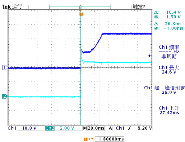
Figure 8, Boot delay time (Iout = 30A)
