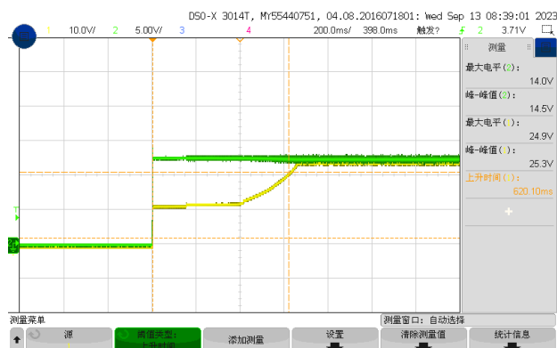
Figure 8, Boot delay time (Iout = 40A)
