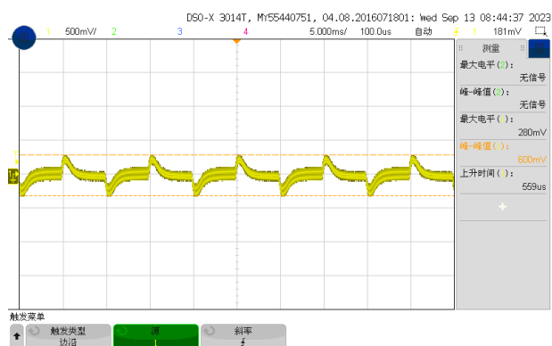
Figure 4, 25% - 50% load dynamic
