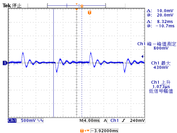
Figure 4, 25% - 50% load dynamic
