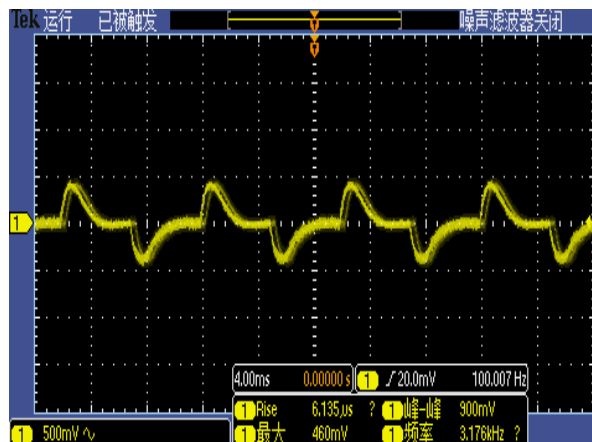
Figure 5, 50% - 75% load dynamic
