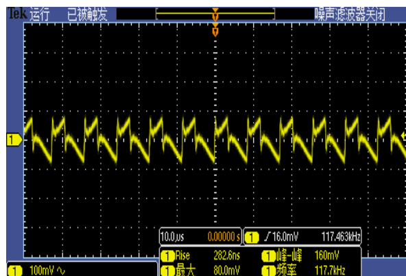
Figure 7, Output ripple & noise ( I_{out} = 10\text{A} )
