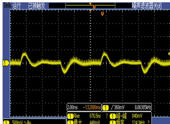
Figure 5, 50% - 75% load dynamic
