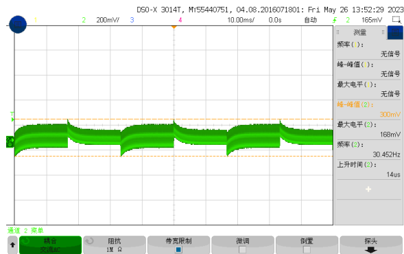
Figure 4, 25% - 50% load dynamic
