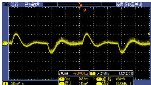
Figure 4, 25% - 50% load dynamic
