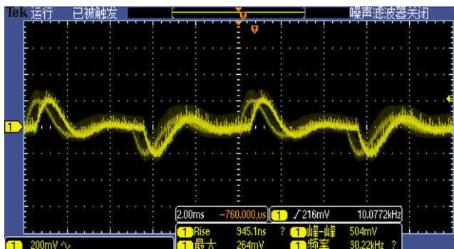
Figure 5, 50% - 75% load dynamic
