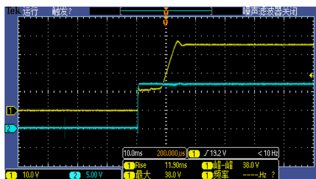
Figure 6, Output voltage established ( I_{out} = 1\text{A} )
