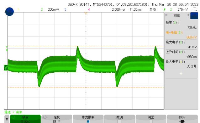
Figure 5, 50% - 75% load dynamic
