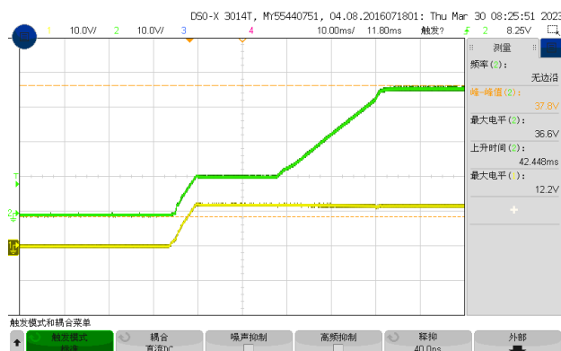
Figure 8, Boot delay time (Iout = 20A)
