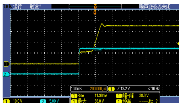
Figure 6, Output voltage established ( I_{out} = 2\text{A} )
