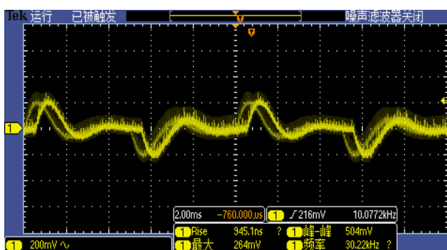
Figure 5, 50% - 75% load dynamic
