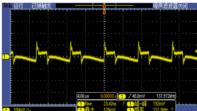
Figure 7, Output ripple & noise ( I_{out} = 2\text{A} )
