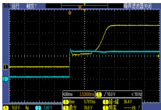
Figure 6, Output voltage established (Iout = 5A)
