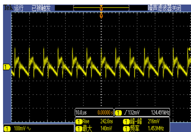
Figure 7, Output ripple & noise (Iout = 5A)
