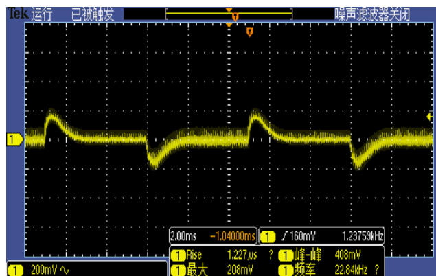
Figure 4, 25% - 50% load dynamic
