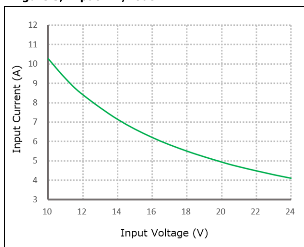
Figure 3, Input V-I, I_{out}=2\text{A}
