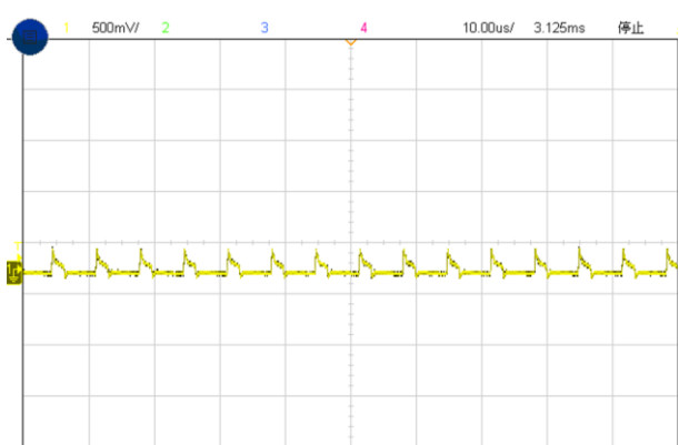
Figure 7, Output ripple & noise ( I_{out} = 2\text{A} )
