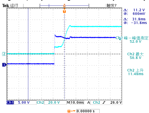
Figure 6, Output voltage established ( I_{out} = 4\text{A} )
