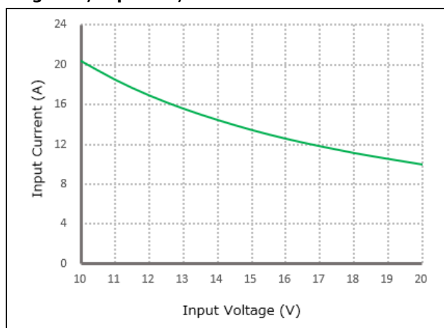
Figure 3, Input V-I, Iout=4A
