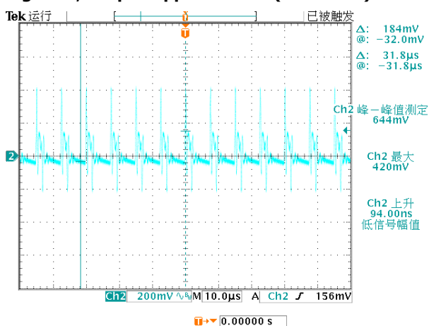
Figure 7, Output ripple & noise ( I_{out} = 4\text{A} )
