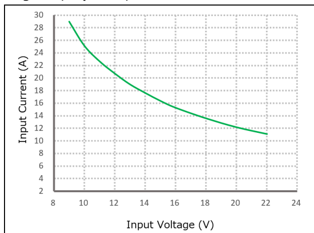
Figure 3, Input V-I, I_{out}=5\text{A}
