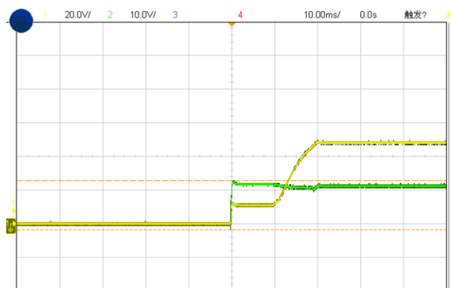
Figure 6, Output voltage established ( I_{out} = 5\text{A} )
