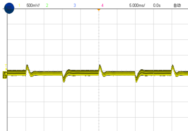
Figure 5, 50% - 75% load dynamic
