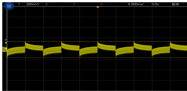
Figure 4, 25% - 50% load dynamic
