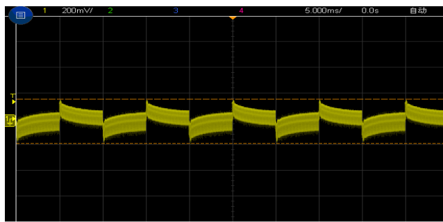
Figure 5, 50% - 75% load dynamic
