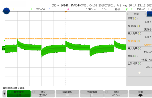
Figure 5, 50% - 75% load dynamic
