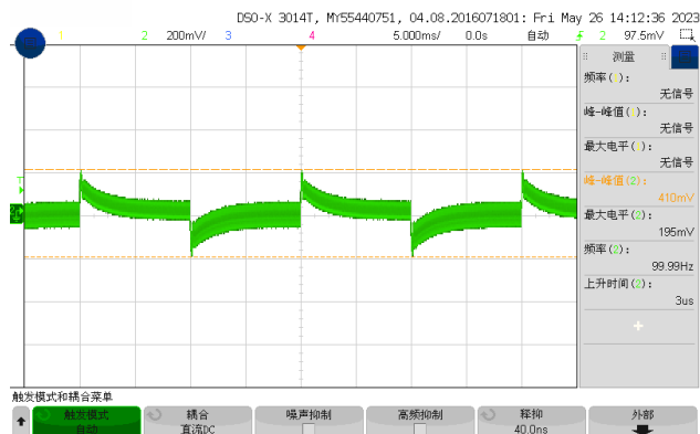
Figure 4, 25% - 50% load dynamic
