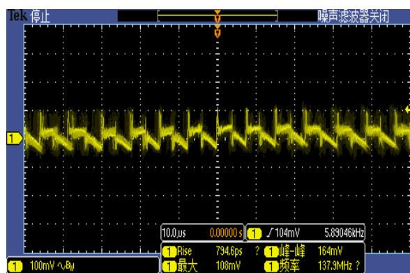
Figure 7, Output ripple & noise ( I_{out} = 3\text{A} )
