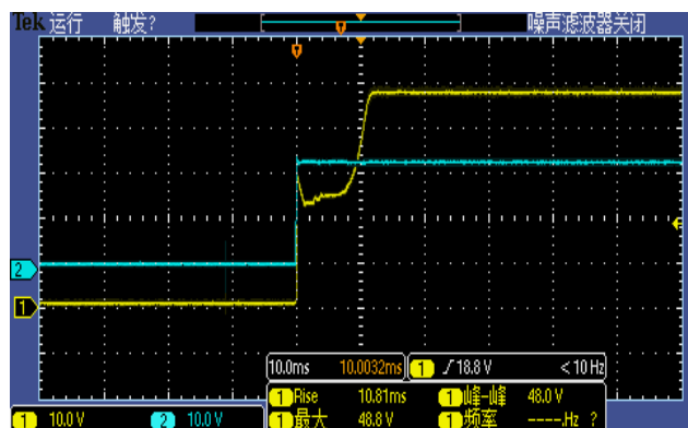
Figure 6, Output voltage established ( I_{out} = 3\text{A} )
