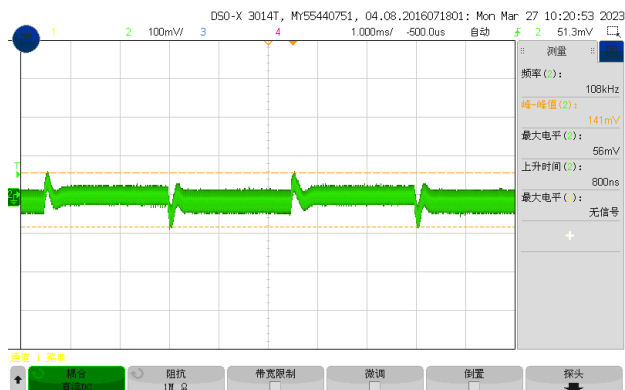
Figure 4, 25% - 50% load dynamic
