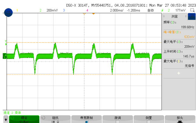
Figure 4, 25% - 50% load dynamic
