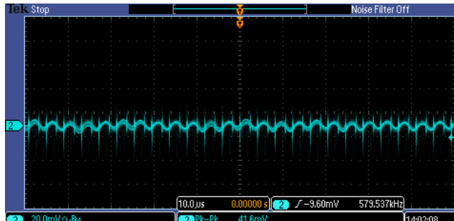
Figure 7, Output ripple & noise ( I_{out} = 8\text{A} )
