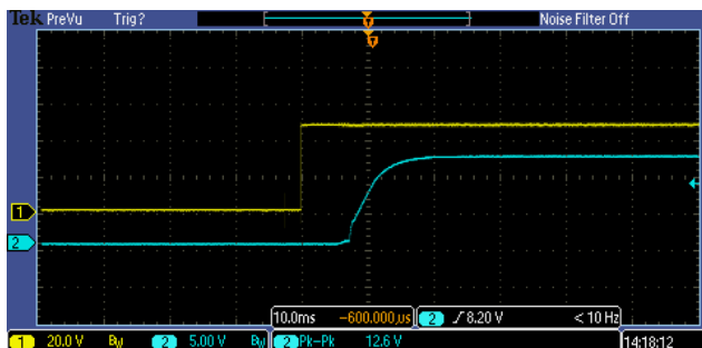
Figure 6, Output voltage established ( I_{out} = 8\text{A} )
