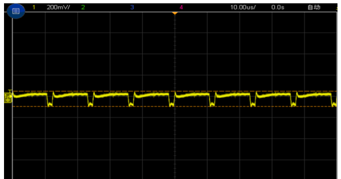
Figure 7, Output ripple & noise ( I_{out} = 30\text{A} )
