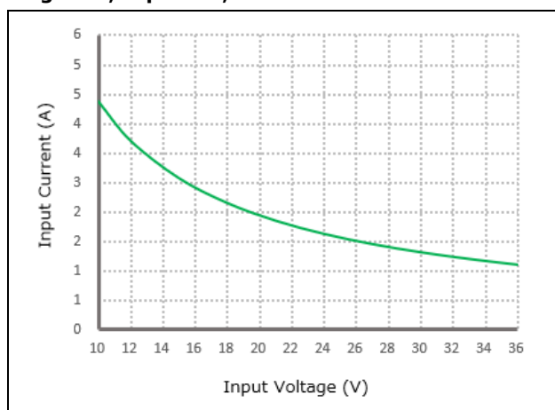
Figure 3, Input V-I, Iout=3A
