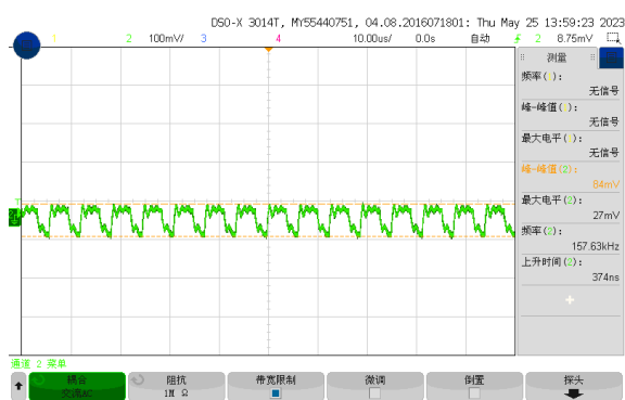
Figure 7, Output ripple & noise (Iout = 5A)
