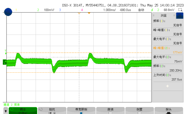
Figure 4, 25% - 50% load dynamic
