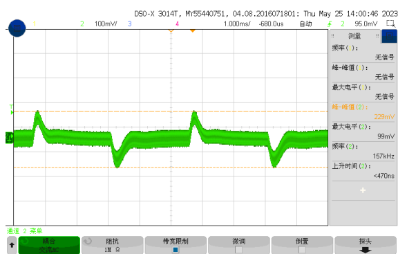
Figure 5, 50% - 75% load dynamic
