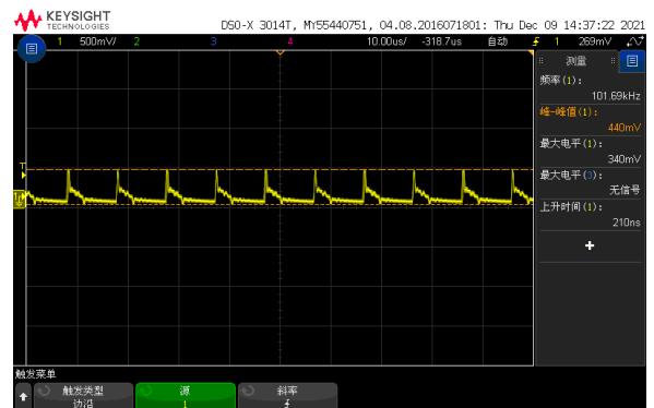
Figure 7, Output ripple & noise ( I_{out} = 2\text{A} )
