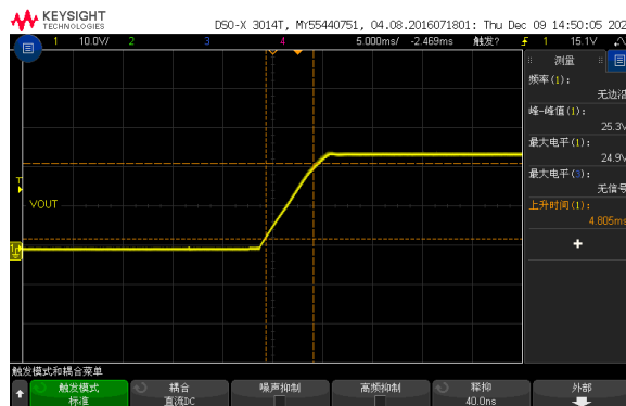
Figure 6, Output voltage established ( I_{out} = 2\text{A} )
