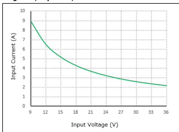
Figure 3, Input V-I, I_{out}=3\text{A}
