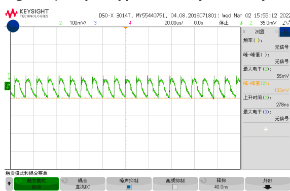
Figure 7, Output ripple & noise (Iout = 3A)
