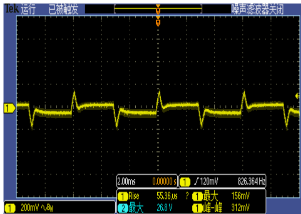
Figure 4, 25% - 50% load dynamic
