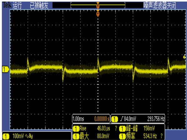
Figure 4, 25% - 50% load dynamic
