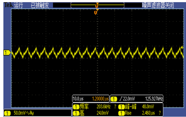
Figure 7, Output ripple & noise ( I_{out} = 20\text{A} )
