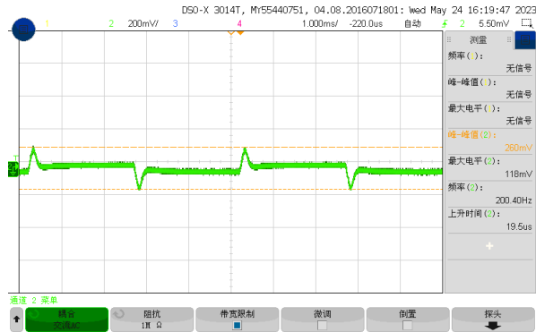
Figure 4, 25% - 50% load dynamic
