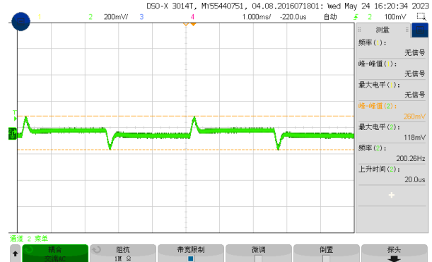
Figure 5, 50% - 75% load dynamic
