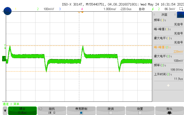
Figure 4, 25% - 50% load dynamic
