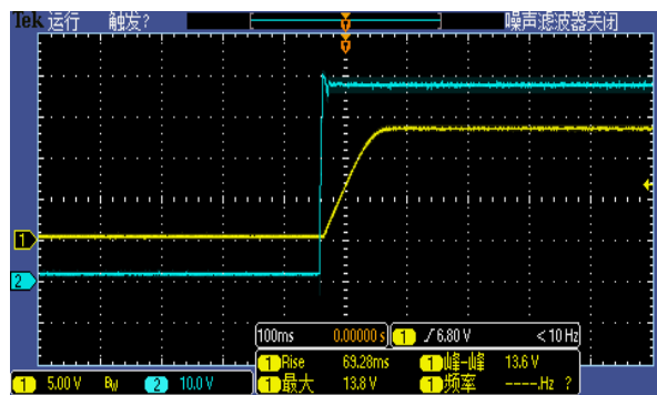
Figure 6, Output voltage established ( I_{out} = 15\text{A} )
