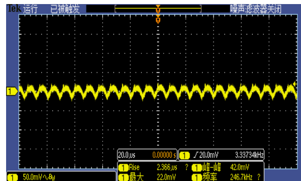
Figure 7, Output ripple & noise ( I_{out} = 15\text{A} )
