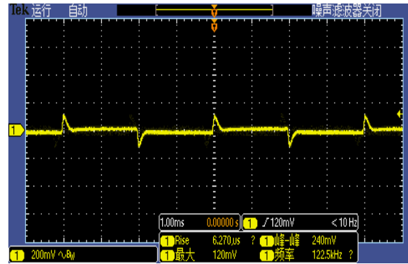
Figure 5, 50% - 75% load dynamic
