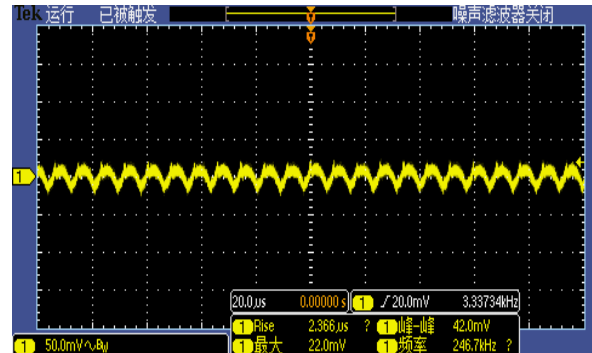
Figure 7, Output ripple & noise ( I_{out} = 20\text{A} )
