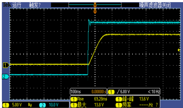
Figure 6, Output voltage established ( I_{out} = 20\text{A} )
