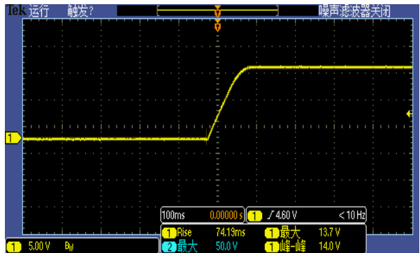
Figure 6, Output voltage established (Iout = 50A)
