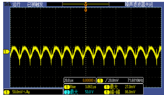
Figure 7, Output ripple & noise (Iout = 50A)
