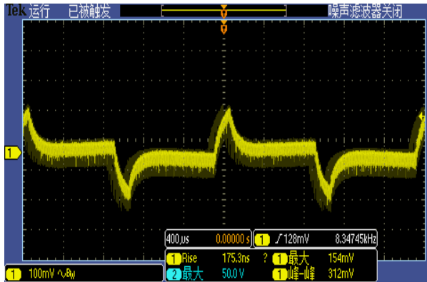
Figure 4, 25% - 50% load dynamic
